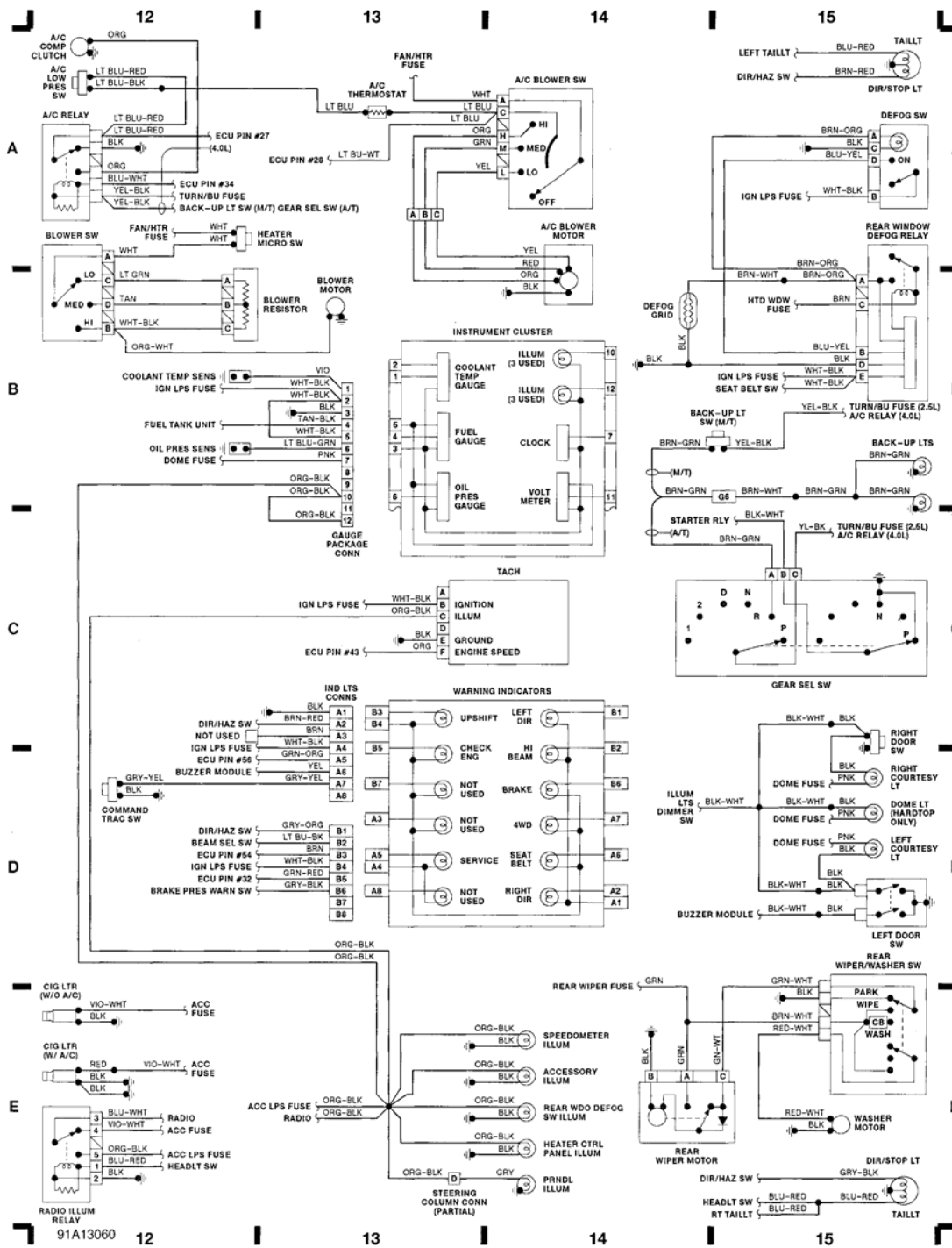
Fig. 4: Multi-Function, Instrument Cluster & Taillights (Grid 12-15)
